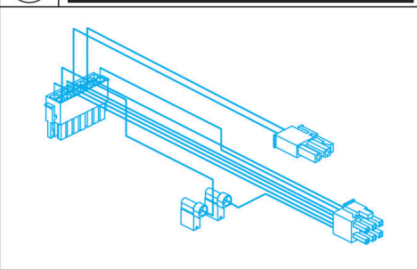
E1 Controller Interface Harness
