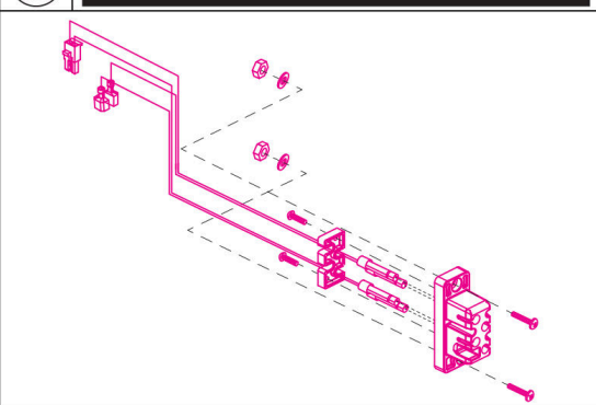
D1 Controller/Motor/Brake Connector
