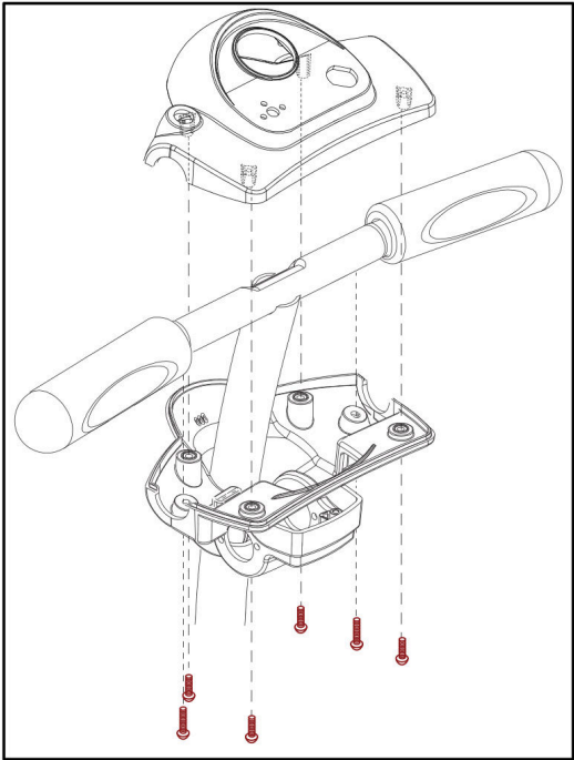
A1 Top Console, LED Voltmeter Assy (Includes B1,C1, & D1)
