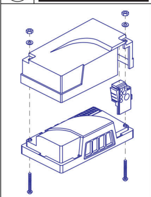
C1 Battery/Controller Connector Assy
