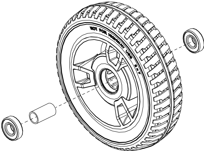
A1 Complete Wheel Assembly
