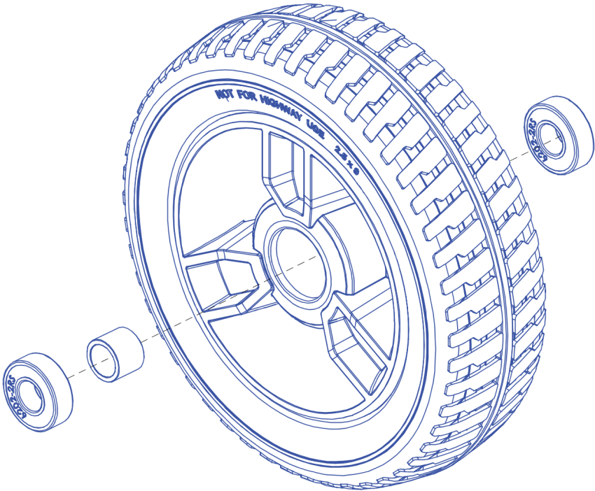
A1 Complete Wheel Assembly
