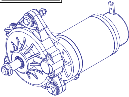
A1 Left Motor Assembly
