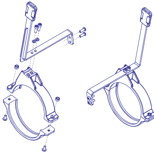
C1 Freewheel Lever Assembly
